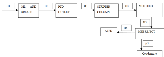
Fig 3: Flowchart for HTDS Waste
