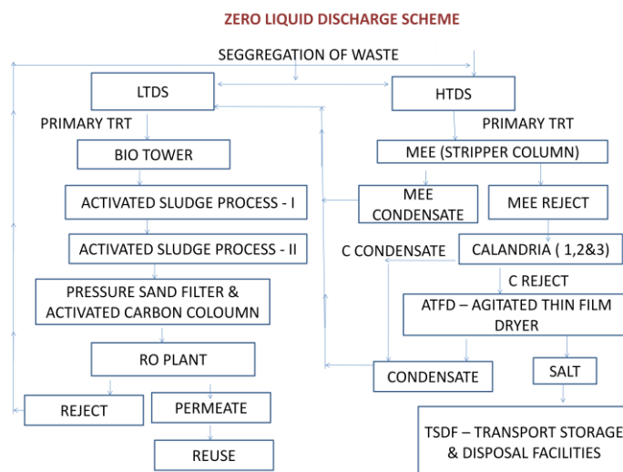
Fig 1: Flowchart Representing Treatment of Waste Water done on the basis of condition 1 and 2
