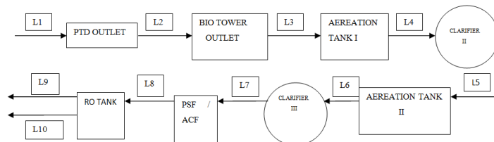
Fig 2: Flowchart for LTDS Waste
