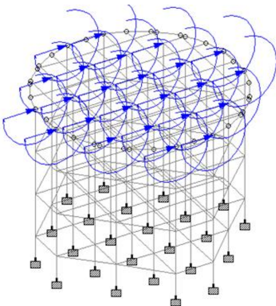
Fig. 3- Wind load on staging
