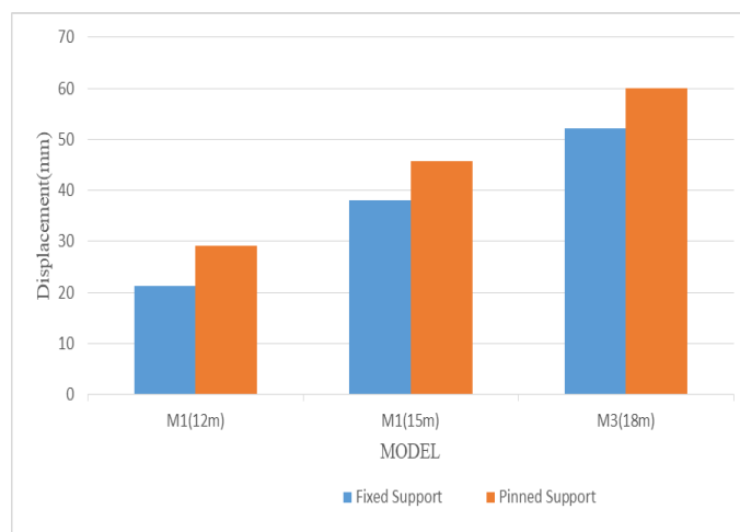
Fig.8- Disp. in zone III Vs zone V
