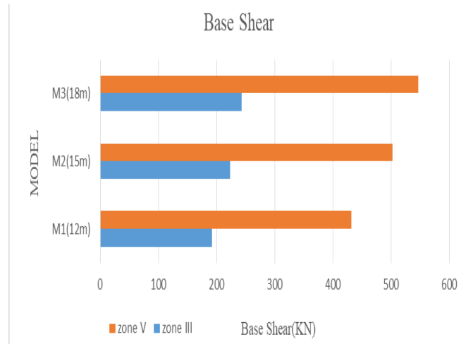
Fig.6- Base Shear in zone III Vs Zone V
