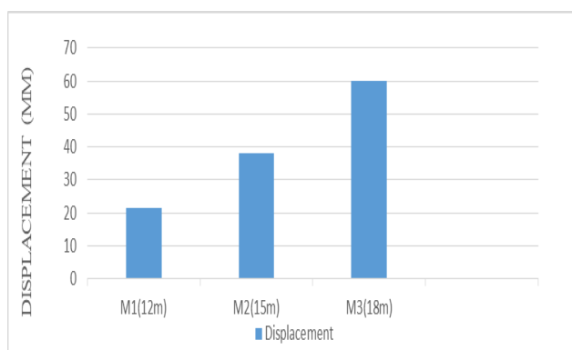
Fig. 5- Height of the tank Vs Displacement
