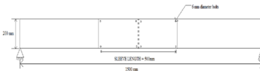
FIGURE 5. SCHEMATIC REPRESENTATION OF SLEEVED CONNECTION
