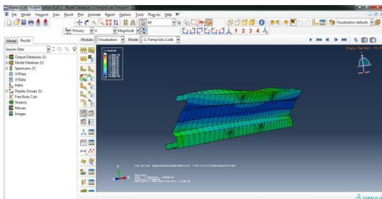
FIGURE 11. STRESS DISTRIBUTION (TYPE 1)
