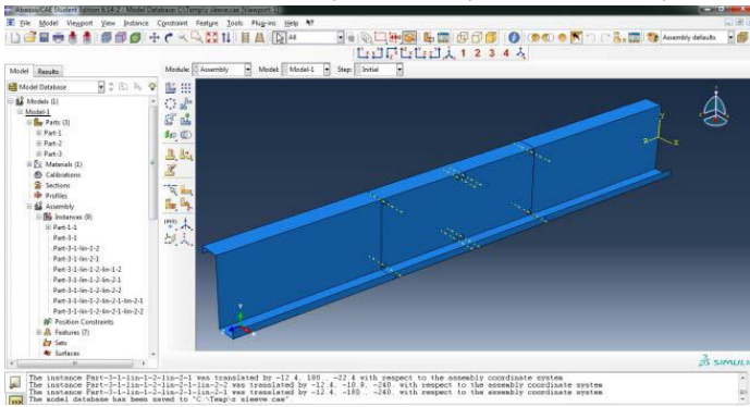
FIGURE 7. MODEL ASSEMBLY FOR Z SECTION SLEEVED CONNECTION
