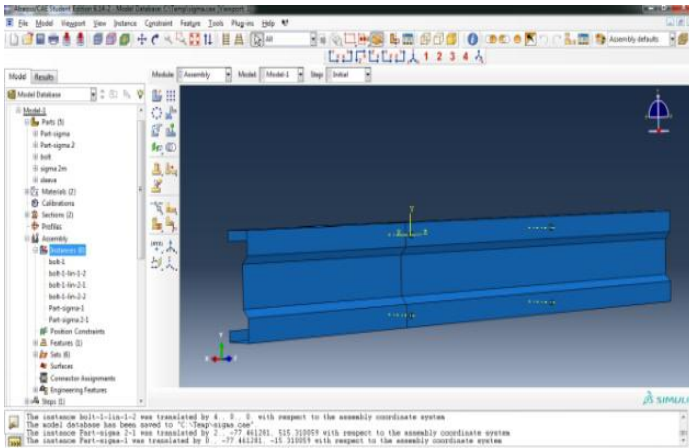
FIGURE 8. MODEL ASSEMBLY FOR SIGMA SECTION LAPPED CONNECTION
