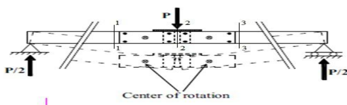
FIGURE 12 CENTRE OF ROTATION FOR SLEEVED CONNECTION
