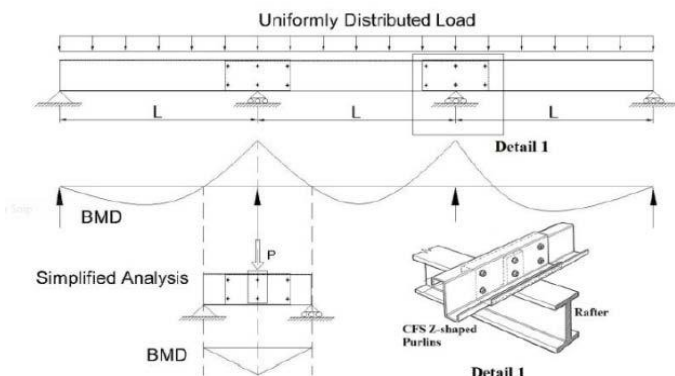
FIGURE 3. SIMPLIFIED ANALYSIS FOR LAPPED CONNECTION
