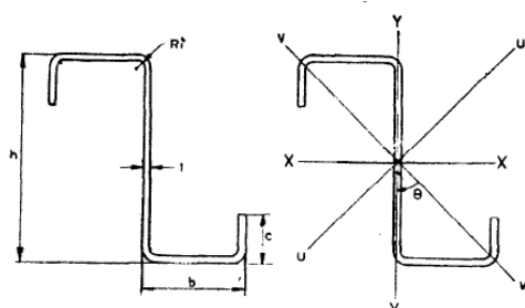
FIGURE 1 . Z SECTION AS PER IS:811-1987
