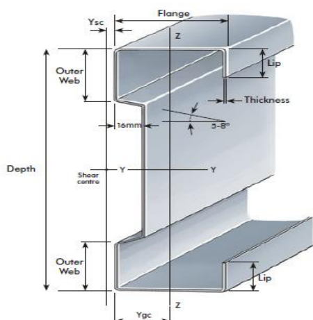
FIGURE 2. SIGMA SECTION BASED ON EUROCODE
