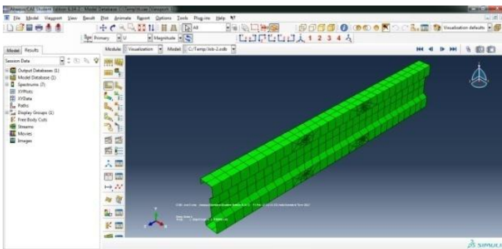
FIGURE 10. MESHING OF MODEL (TYPE 3)
