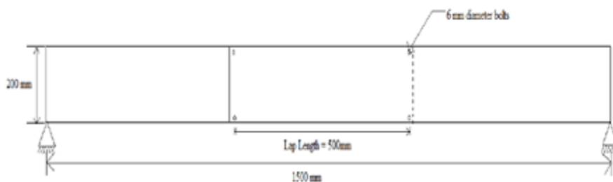
FIGURE 4. SCHEMATIC REPRESENTATION OF LAPPED CONNECTION
