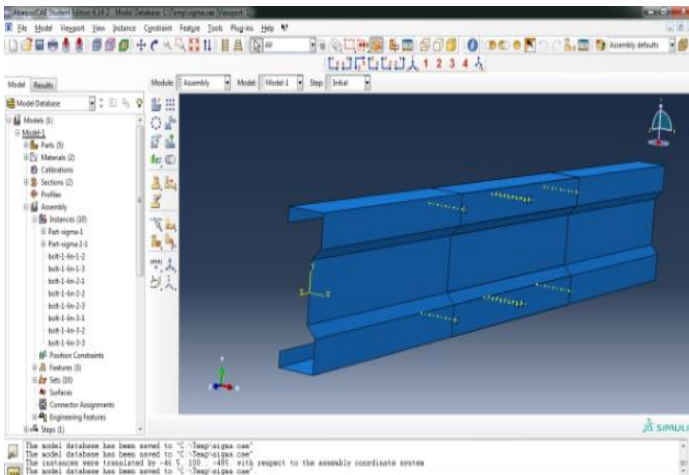
FIGURE 9. MODEL ASSEMBLY FOR SIGMA SECTION SLEEVED CONNECTION
