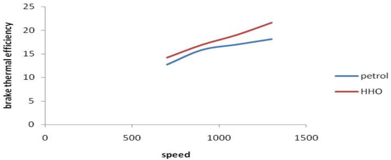
Graph 9. Variation of speed with brake thermal efficiency for petrol and HHO gas
