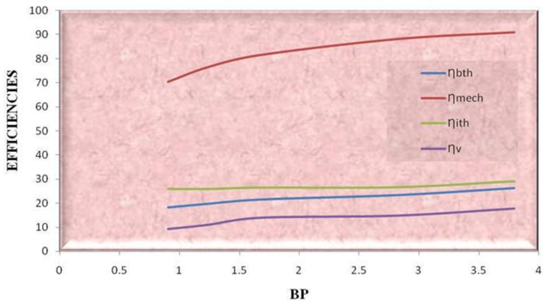
Graph 8. Variation of Brake Power (BP) with Efficiencies at 1300 rpm
