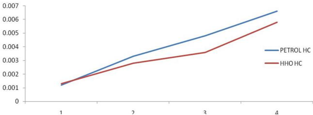
Graph 10. Variation of flow rate with hydrocarbon (HC) emissions for petrol and HHO gas
