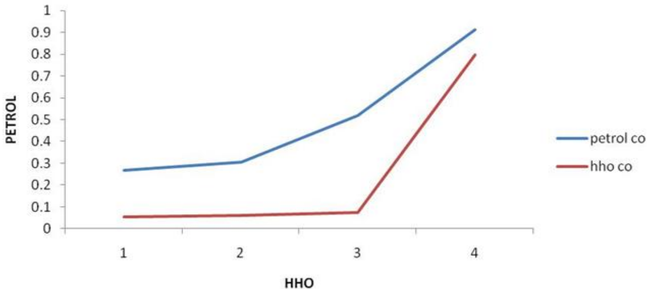
Graph 11. Variation of flow rate with carbon monoxide (CO) emissions for petrol and HHO gas
