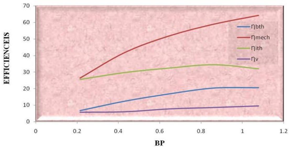
Graph 5. Variation of Brake Power (BP) with Efficiencies at 700 rpm
