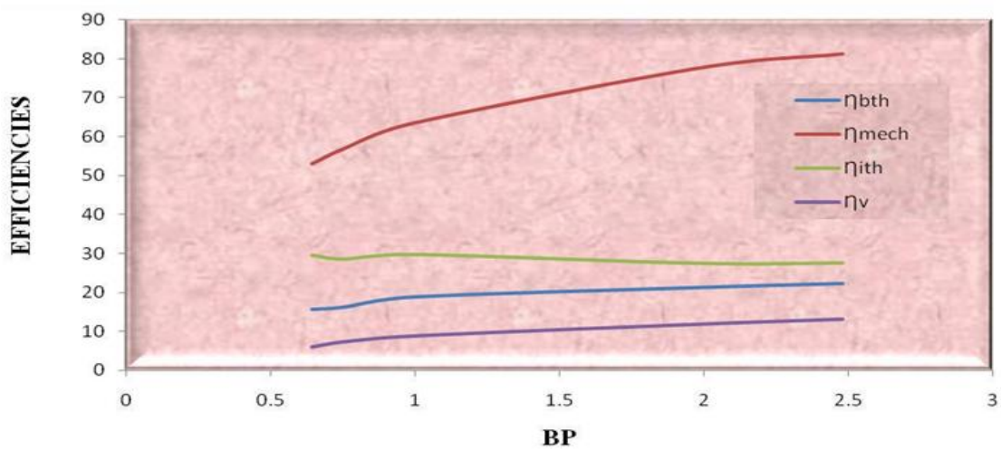
Graph 6. Variation of Brake Power (BP) with Efficiencies at 900 rpm
