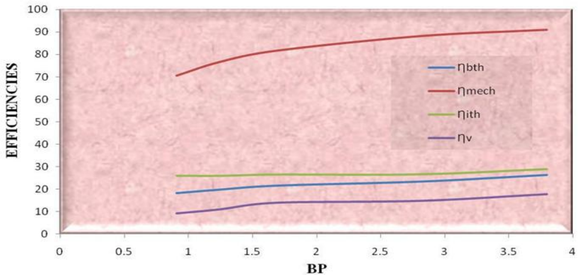
Graph 7. Variation of Brake Power (BP) with Efficiencies at 1100 rpm
