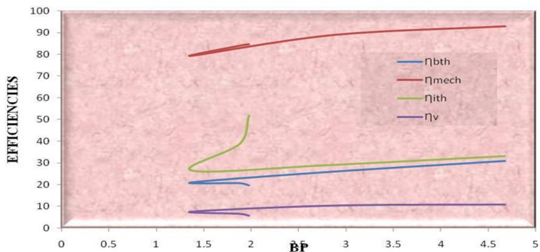
Graph 3. Variation of Brake Power (BP) with Efficiencies at 1100 rpm
