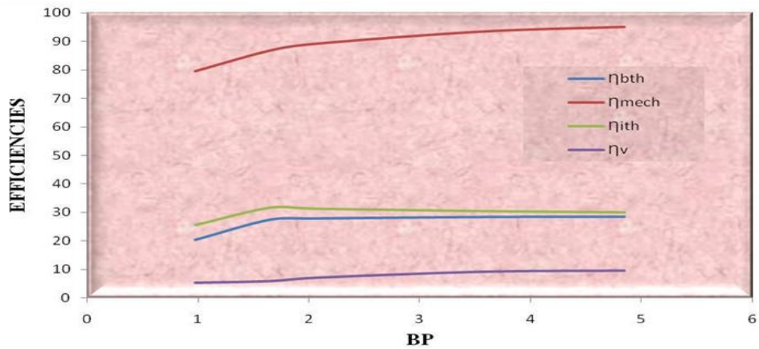
Graph 4. Variation of Brake Power (BP) with Efficiencies at 1300 rpm
