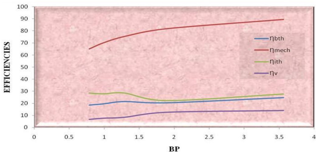
Graph 2. Variation of Brake Power (BP) with Efficiencies at 900 rpm
