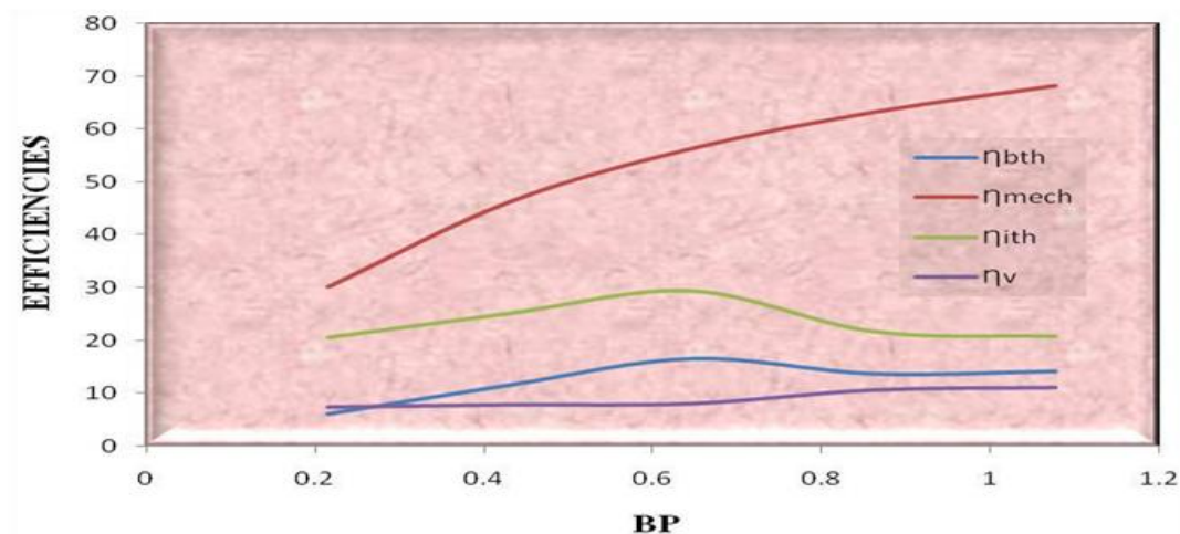
Graph 1. Variation of Brake Power (BP) with Efficiencies at 700 rpm
