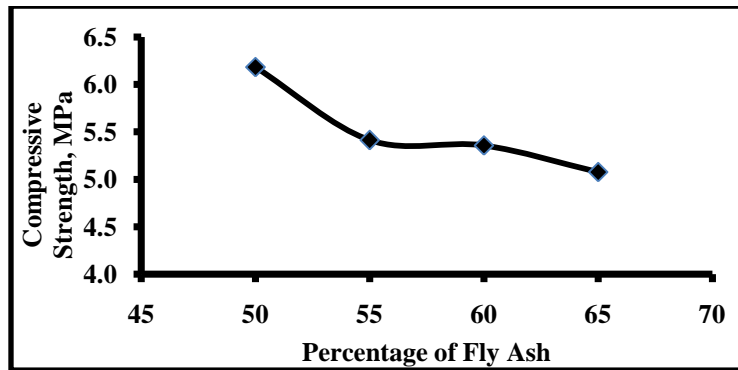
Fig. 5 Variation of Compressive Strength with fly ash content
