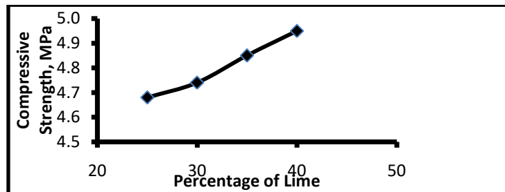
Fig. 6 Variation of Compressive Strength with lime content
