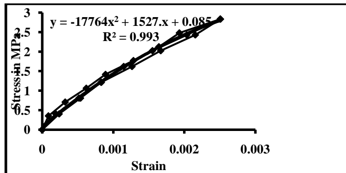
Fig. 9 Modulus of elasticity at 28 days of series H9[50:40:10][Sand]
