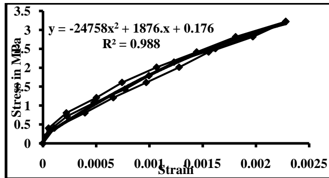
Fig. 8 Modulus of elasticity at 28 days of series H3[55:35:10][QD]
