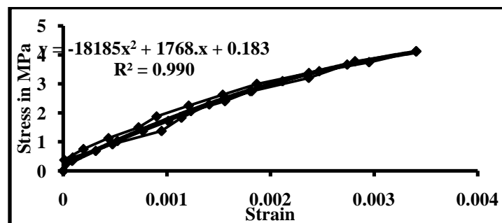
Fig. 7 Modulus of elasticity at 28 days of series H1[50:40:10][QD]
