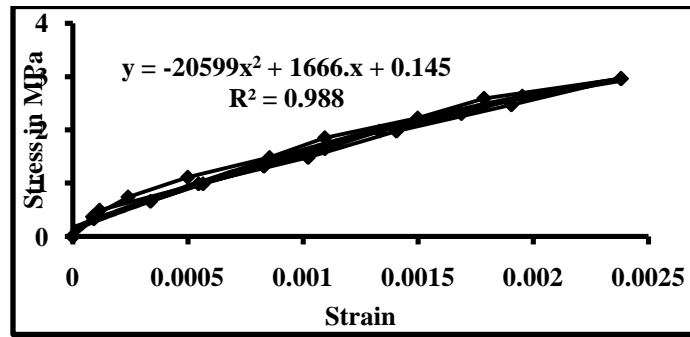
Fig. 8 Modulus of elasticity at 28 days of series H3[55:35:10][QD]
