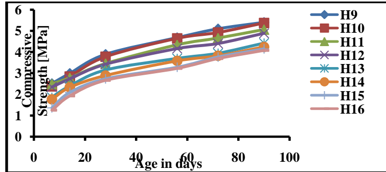
Fig. 2 Variation of Compressive Strength with age with Sand as fine aggregate
