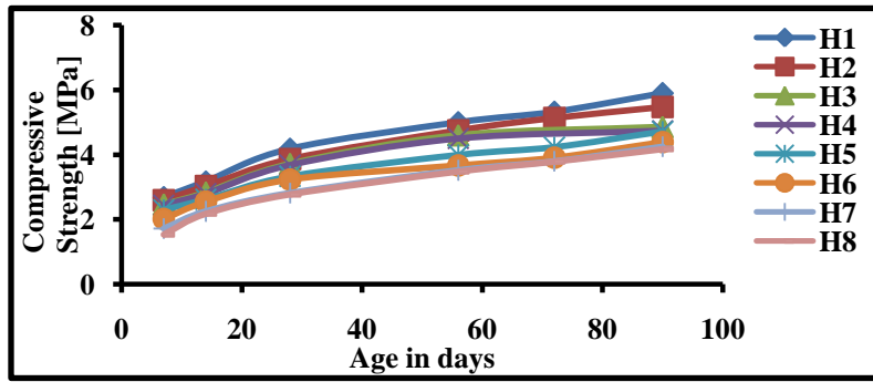
Fig. 1 Variation of Compressive Strength with age with quarry dust as fine aggregate
