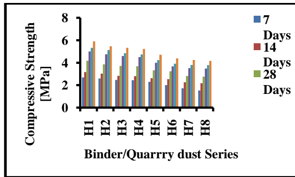
Fig. 3 Compressive Strength of H1 to H8 of Binder/Quarry dust Series for various ages
