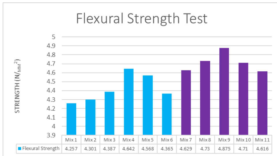
Figure 6. Flexural strength test result of M30 grade of concrete
