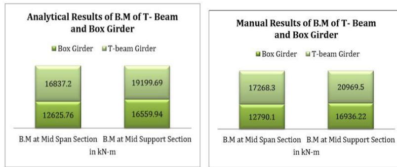
Fig. 4: Manual & Analytical Results of B.M of T- Beam and Box Girder
