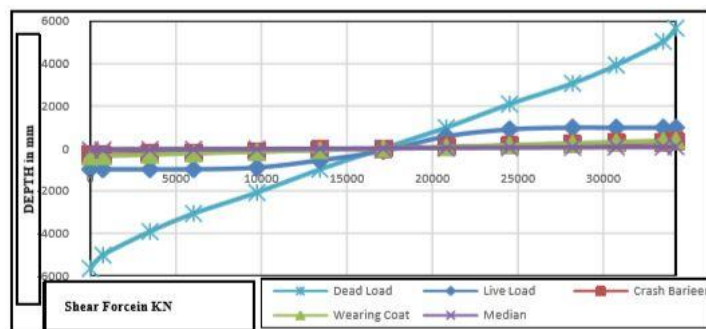
Fig. 3: Shear force diagram for different loadings
