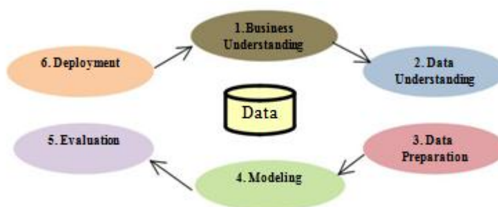
Fig. 1. CRISP-DM methodology
