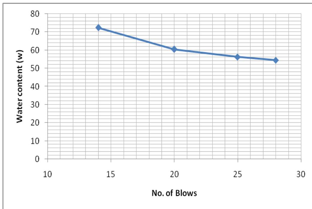
Figure : Liquid limit of parent soil
