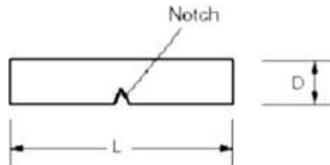
Fig : Dimensions of Impact Test Specimen
