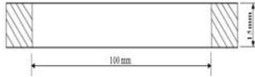
Fig : Dimensions of Flexural Test Specimen
