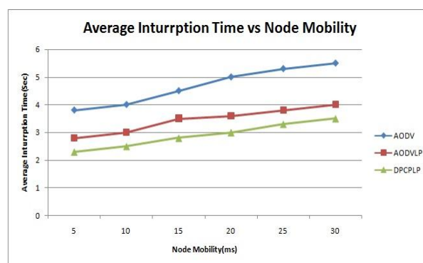
Figure.2 Average Interruption Time Vs Node Velocity
