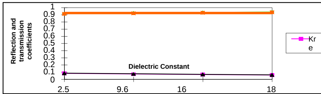
Graph No. 3 Dependence of reflection and transmission coefficients on permittivity
