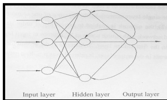
Figure 5: recurrent network
