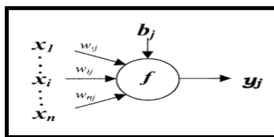
Figure 2: input data
