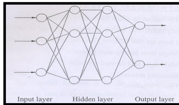
Figure 4: multilayer feed forward network
