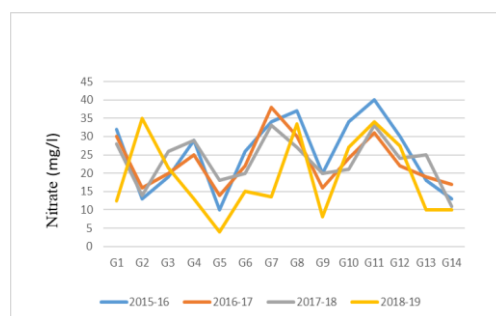
Fig. 18: Temporal variation of Nitrates
