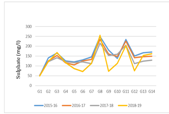
Fig. 16: Temporal variation of Sulphate
