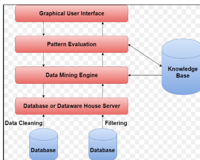
Figure 1: Architectural Components of Data Mining
