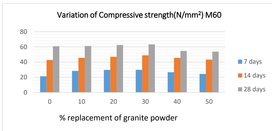
Fig 4: Compressive strength of M60 Concrete (N/mm 2 )
