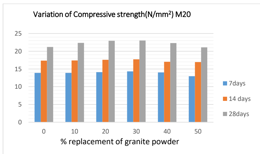
Fig 1: Compressive strength of M20 Concrete (N/mm2)
