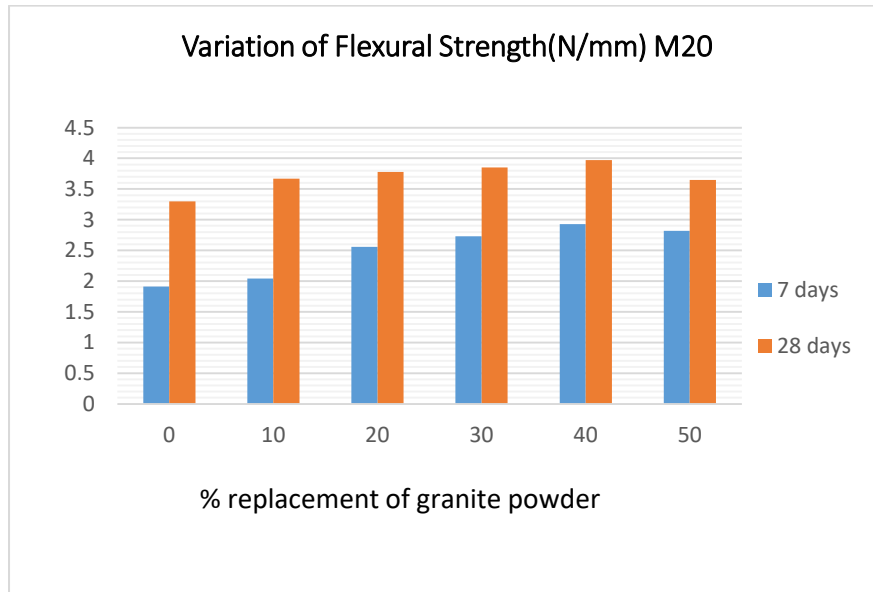
Fig 3: Flexural strength of M20 Concrete (N/mm 2 )
