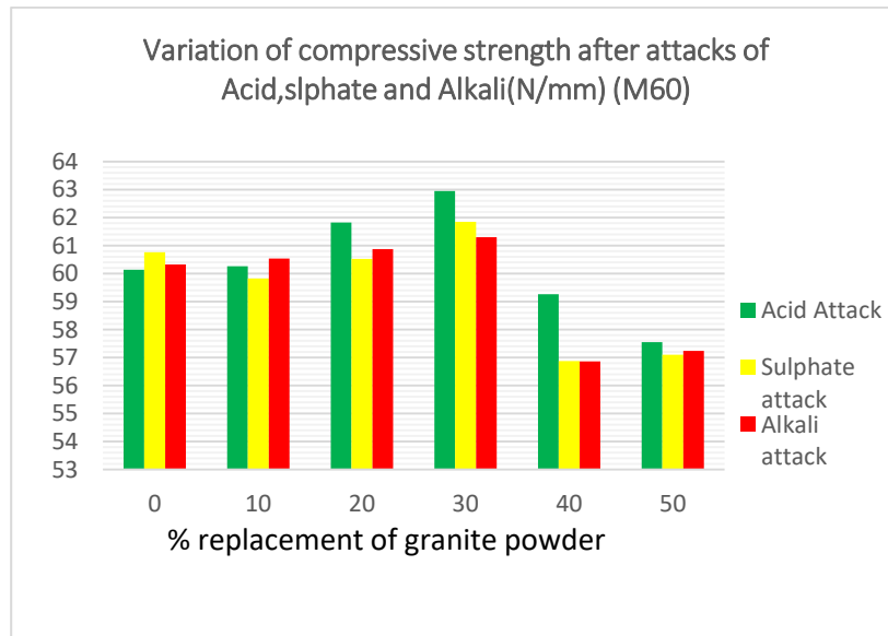
Fig 8: Compressive strength of M60 Concrete
