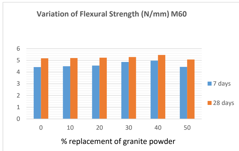
Fig 6: Flexural strength of M60 Concrete (N/mm 2 )
