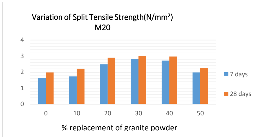
Fig 2: Split Tensile strength of M20 Concrete (N/mm²)
