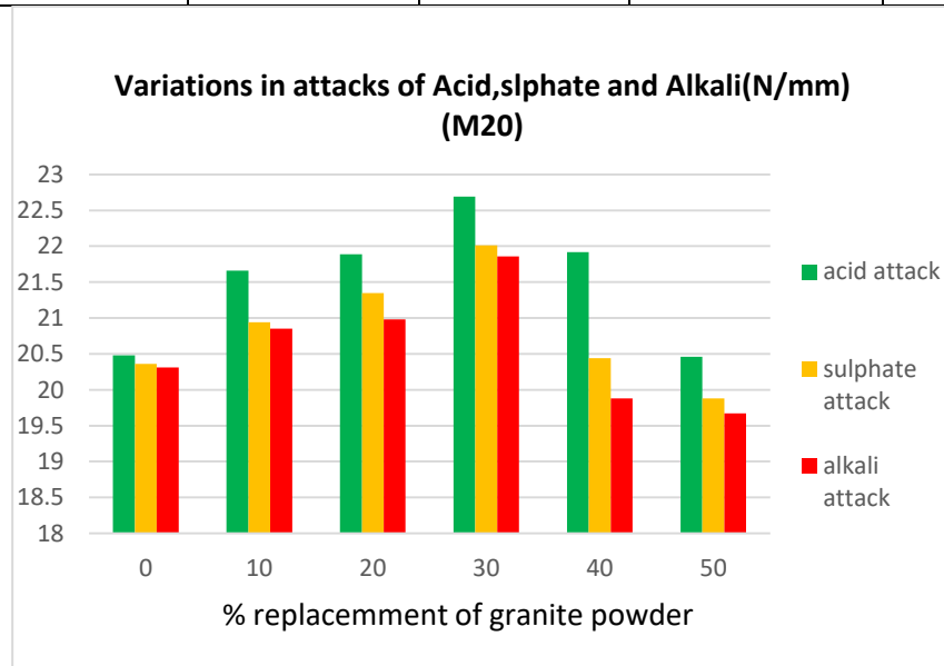
Fig 7: Compressive strength of M20 Concrete (N/mm 2 )
