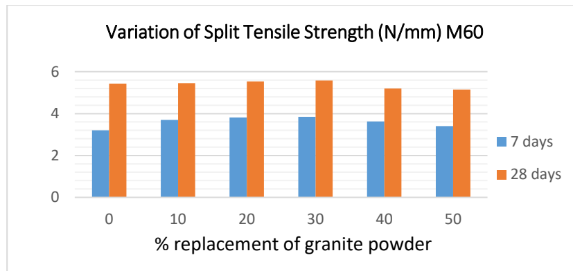
Fig 5: Split Tensile strength of M60 Concrete (N/mm 2 )
