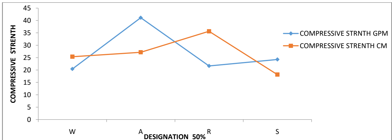
Figure 7.3: correlation between compressive strength and designation of different sand for 50%
