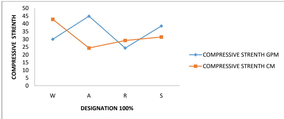
Figure 7.2: correlation between compressive strength and designation of different sand for 100%
