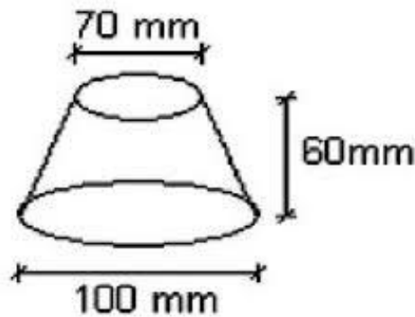
Figure 6.1: Dimensions of mini slump cone (Source: ASTM C 1437:2013)
