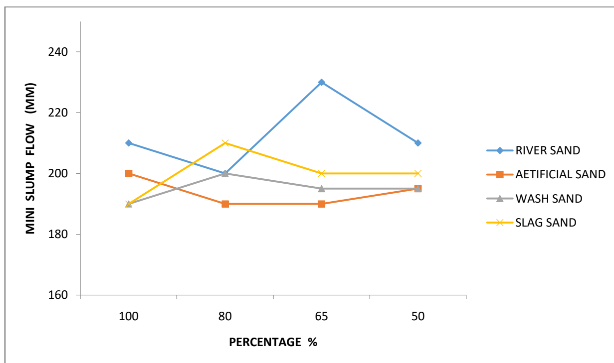
Figure 7.1: correlation between mini slump flow and different percentage of sands for geopolymer mortar
