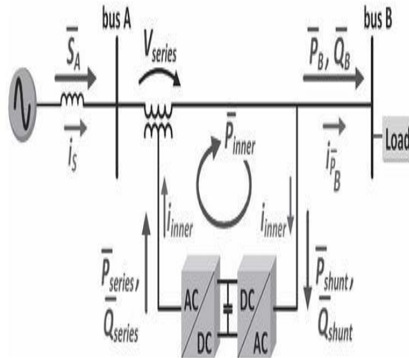
Figure: 4 iUPQC power flow in steady-state
