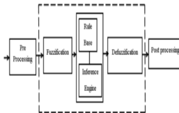
Figure: 5 Fuzzy logic controllers
