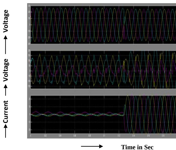
Figure: 8 iUPQC response at no load condition: (a) grid voltages V_A , (b) load voltages V_B , and (c) grid currents.
