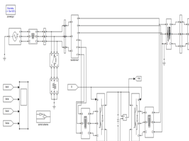
Figure: 9 Simulink circuit for the load currents, grid currents, load voltages and grid voltages at iUPQC transitory response during the connection of a three phase diode rectifier
