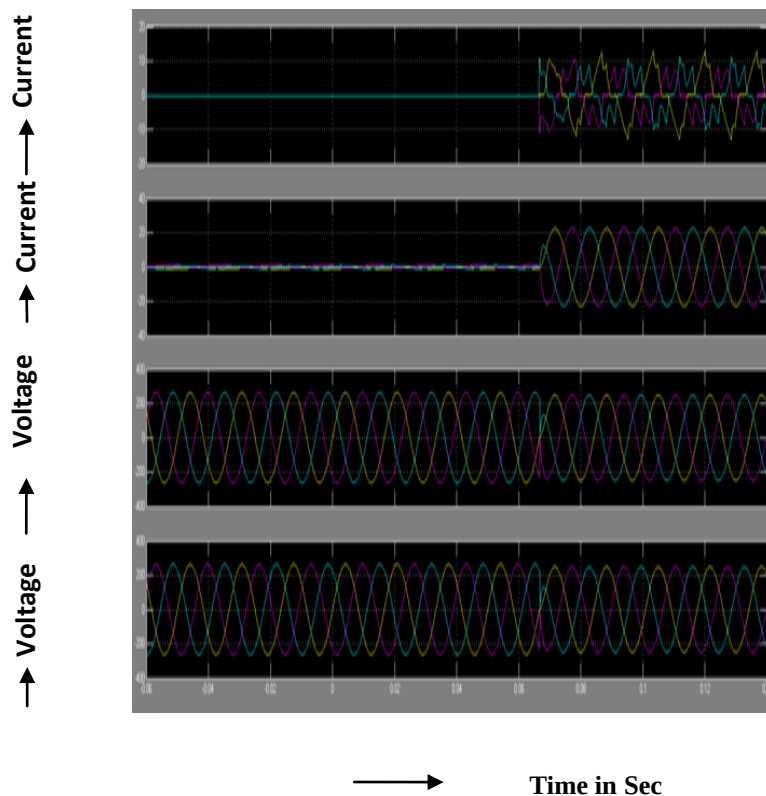
Figure :10 : iUPQC transitory response during the connection of a three phase diode rectifier: (a) load currents, (b) grid currents, (c) load voltages and (d) grid voltages.
