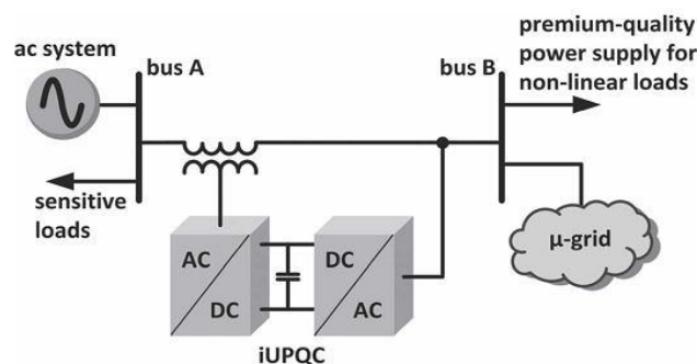
Figure : 1 Block diagram of IUPQC
