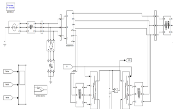
Figure: 7 Simulink circuit for the load voltage, grid voltage and current iUPQC response at no load condition.
