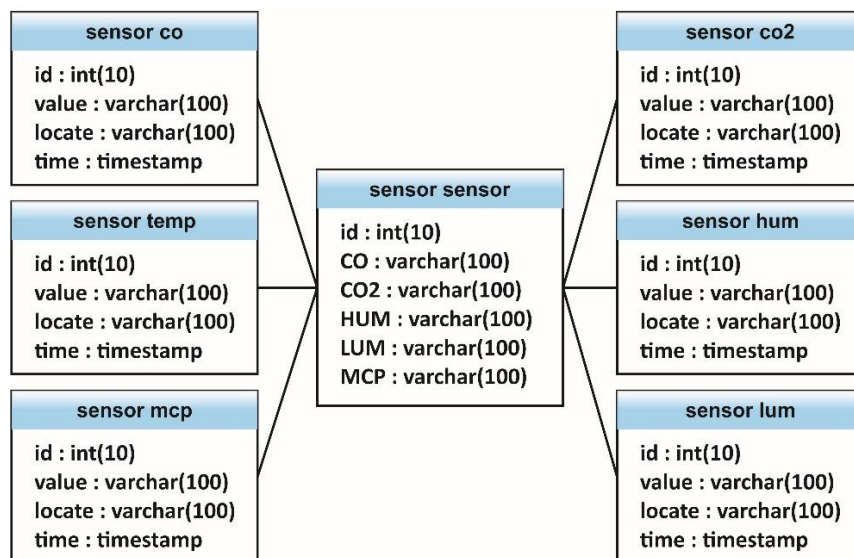
Fig. 10 Relational database
