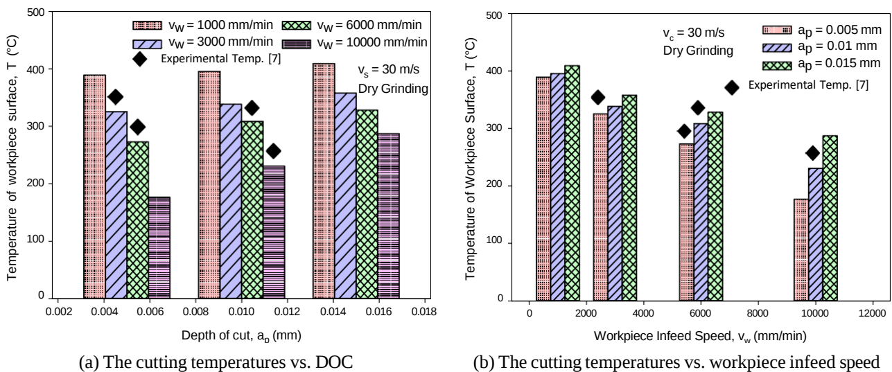
Fig. 11 The effect of grinding conditions on grinding temperature through FEM
