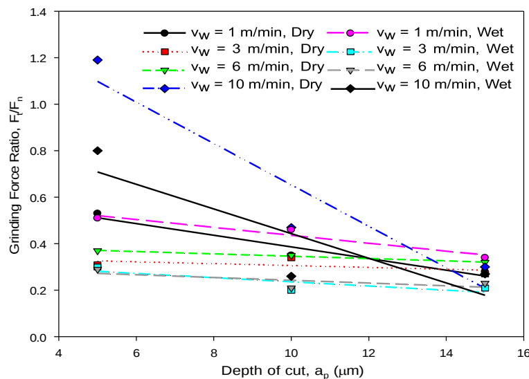
Fig. 5 The effect of DOC and v_w on grinding force ratio F_t/F_n at various cooling conditions
