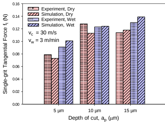
(c) Single-grit tangential force vs. depth of cut
