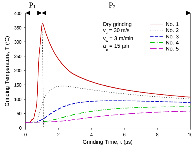
Fig. 10 The temperature profile of five checkpoints
