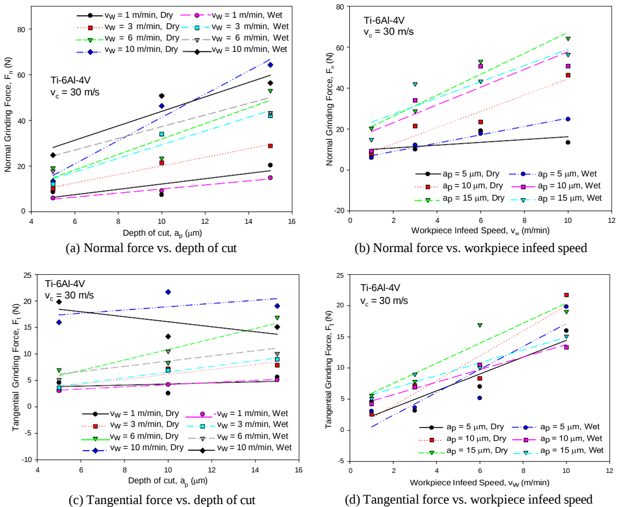
Fig. 4 The influence of DOC and workpiece infeed speed on grinding forces at different cooling conditions
