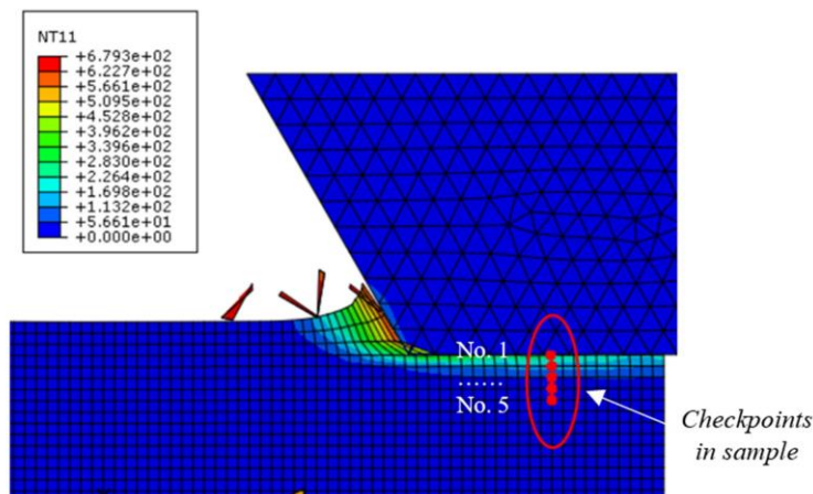
Fig. 9 The simulation of temperature distribution in single-grain grinding
