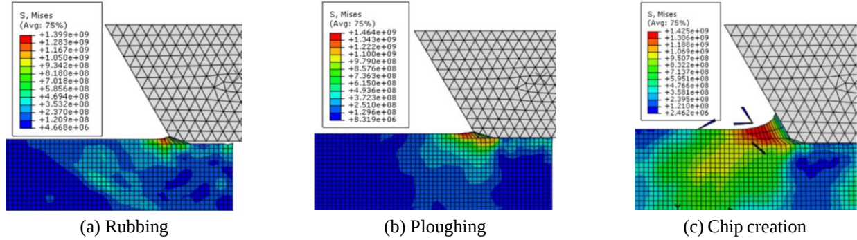
Fig. 7 The simulation of three periods in the single-grain grinding process of Ti-64 alloy
