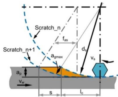
Fig. 3 Grinding operation of a single grain [14]
