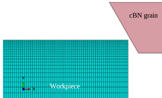
Fig. 2 The 2D FEM model for the grinding process with a single abrasive grain
