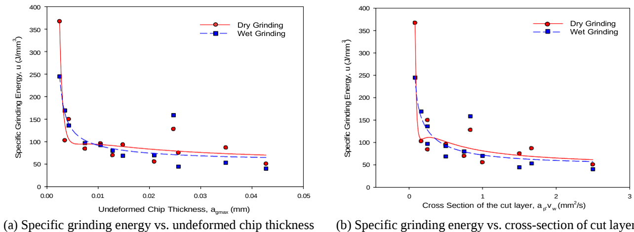
Fig. 6 The effect of undeformed chip thickness and cross-section of the cut layer on the specific grinding energy
