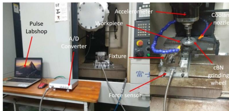
Fig. 1 The setup for the surface grinding experiments
