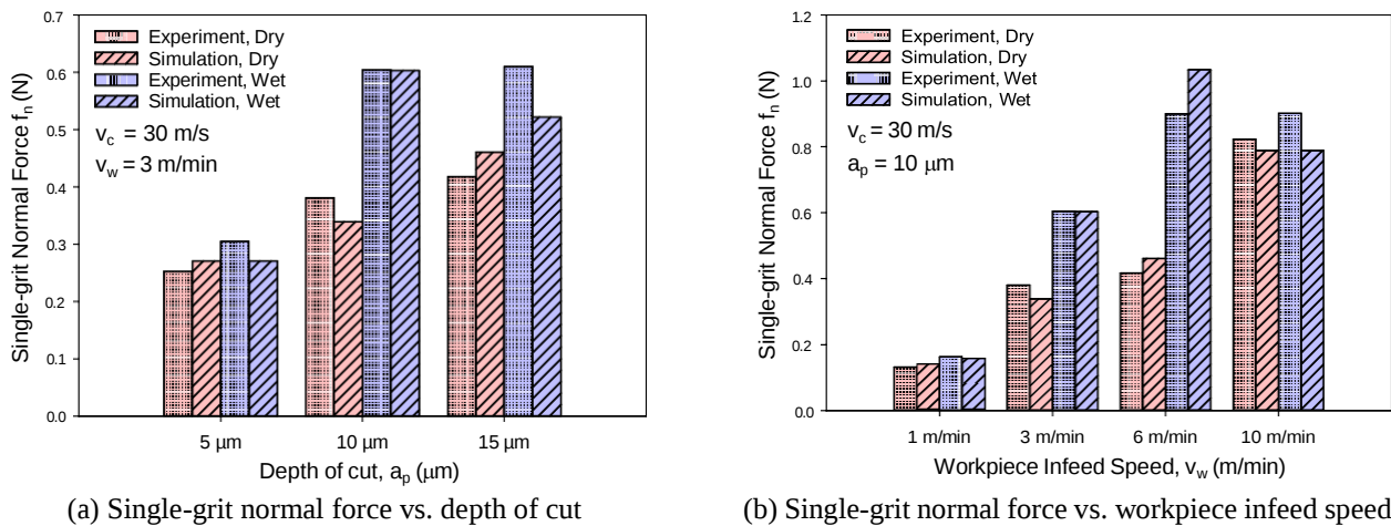
Fig. 8 The comparison of single-grit grinding forces between simulated and experimental results
