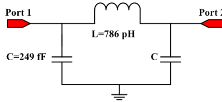
Fig. 4 Schematic of the DUT2 in the S_{21} detection circuit
