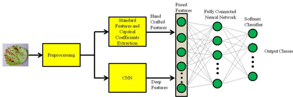
Fig. 4 Framework for feature fusion
