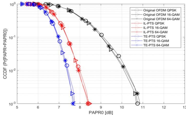
Fig. 7 Comparison the TE-PTS and IL-PTS schemes for various modulation families when N=128
