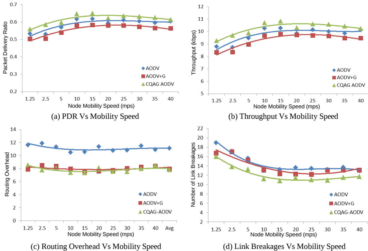
Fig. 6 Performance Analysis of CQAG-AODV for Node Mobility in Sparse Network scenario
