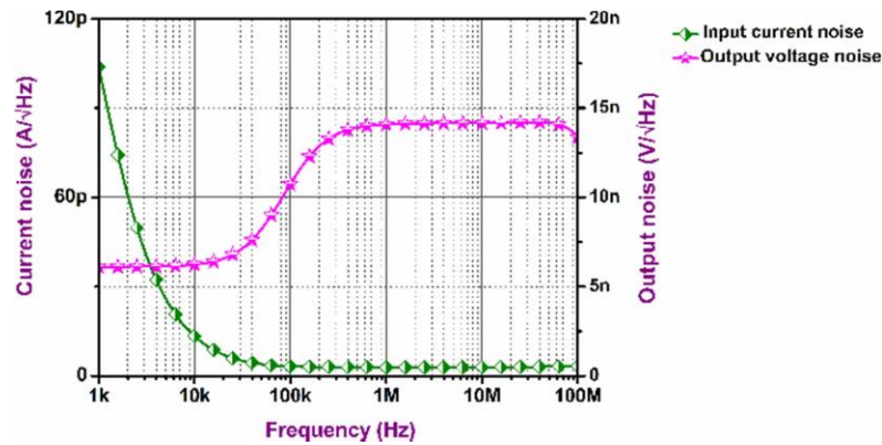
Fig. 24 Output and input referred noise responses of GIS-4
