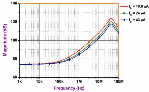
(a) For different I_B
