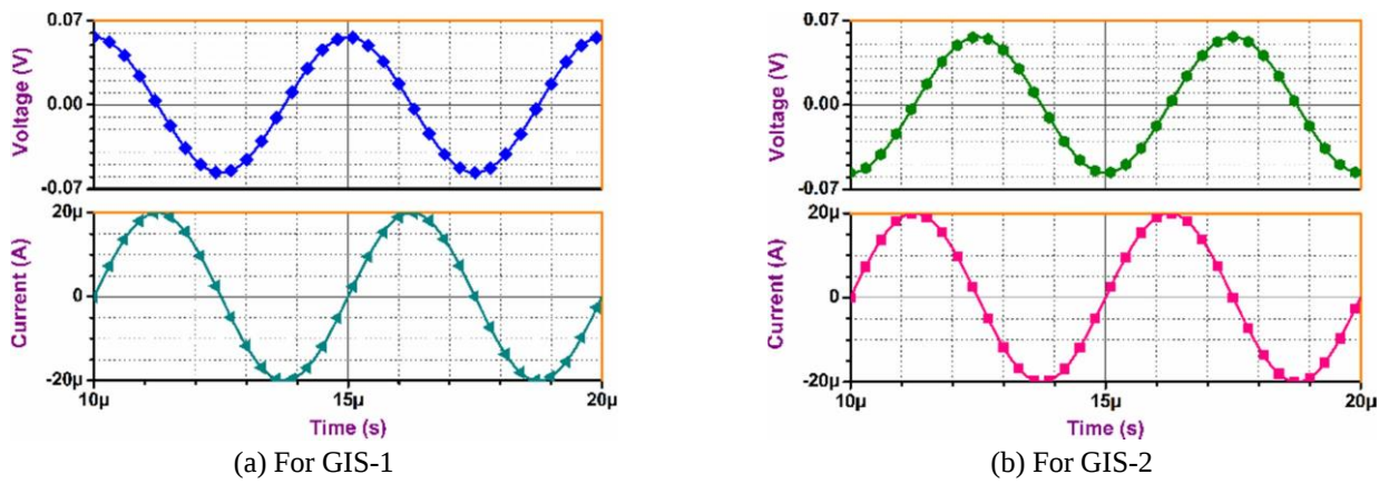
Fig. 7 The transient analysis output
