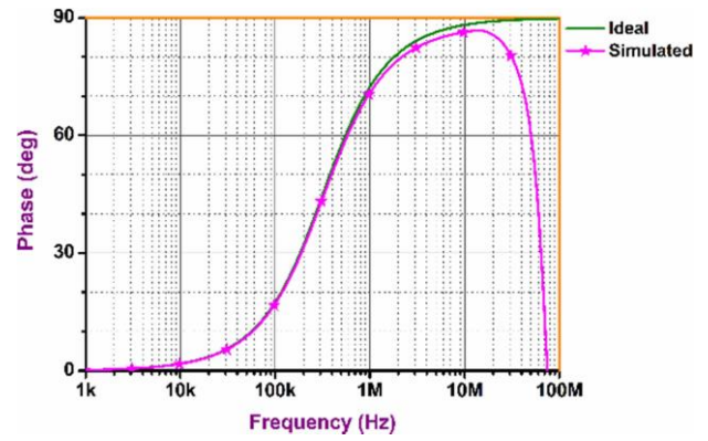
(b) Phase
