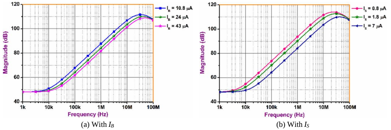
Fig. 9 Variation of impedance magnitude for GIS-2
