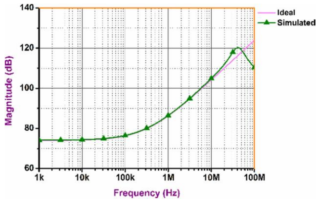
(a) Impedance
