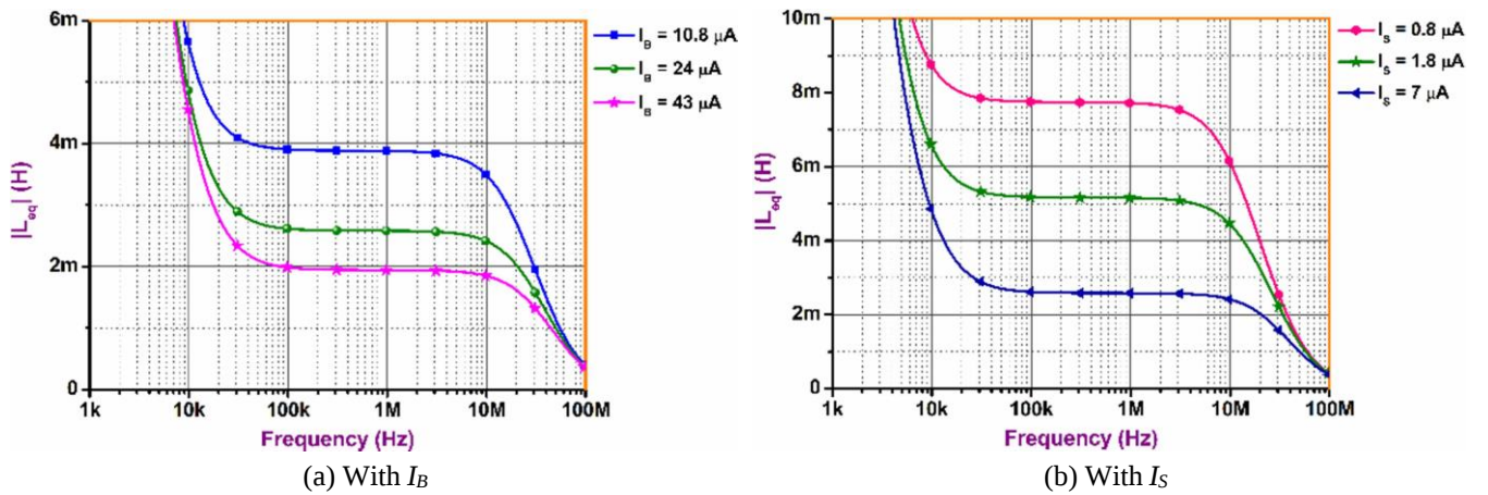
Fig. 11 Variation of inductance for GIS-2
