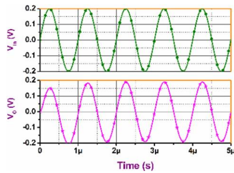
Fig. 27 Transient analysis result of the BP filter
