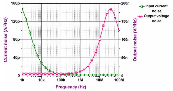
(b) For negative inductor (GIS-2)
