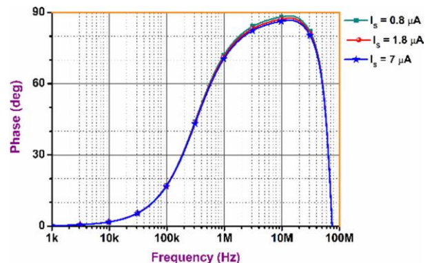
(b) For different I_S
