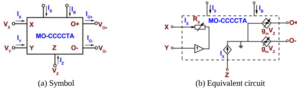
Fig. 1 MO-CCCCTA [30]
