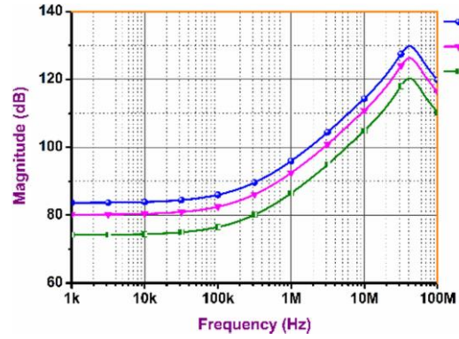
(b) For different I_S
